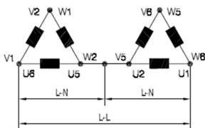
SINGLE PHASE DOUBLE DELTA
